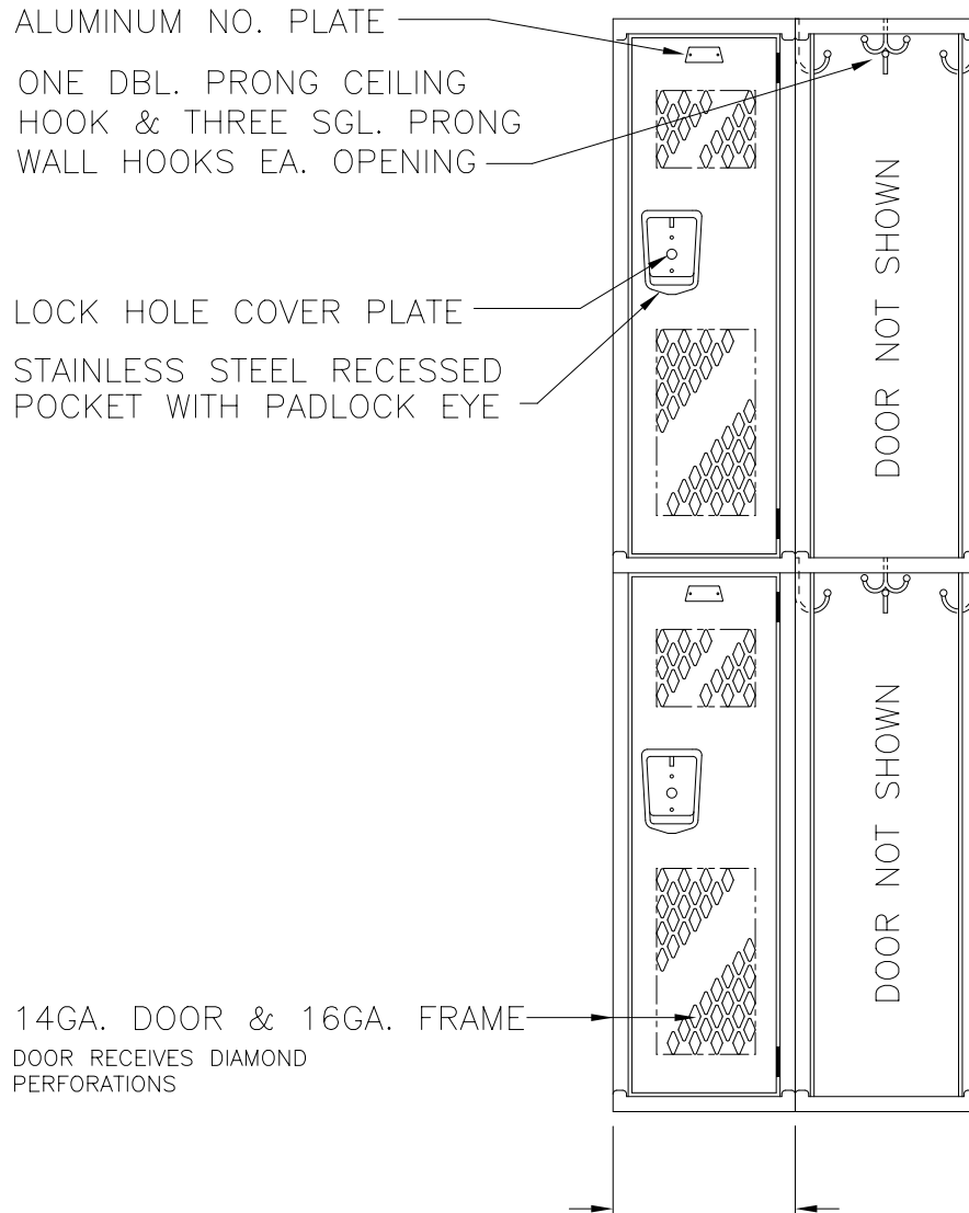
ELEVATION SECTION @ WALL 72" HIGH DOUBLE TIER INVINCIBLE II KNOCKDOWN LOCKER
