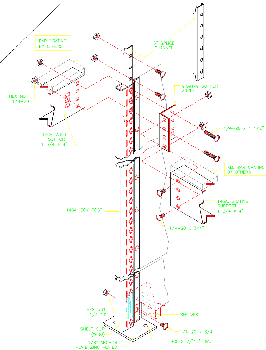
ASSEMBLY DETAIL
