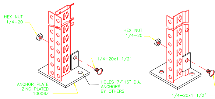
INTERMEDIATE POST
