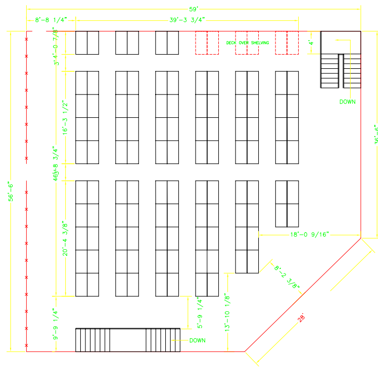
UPPER LEVEL
