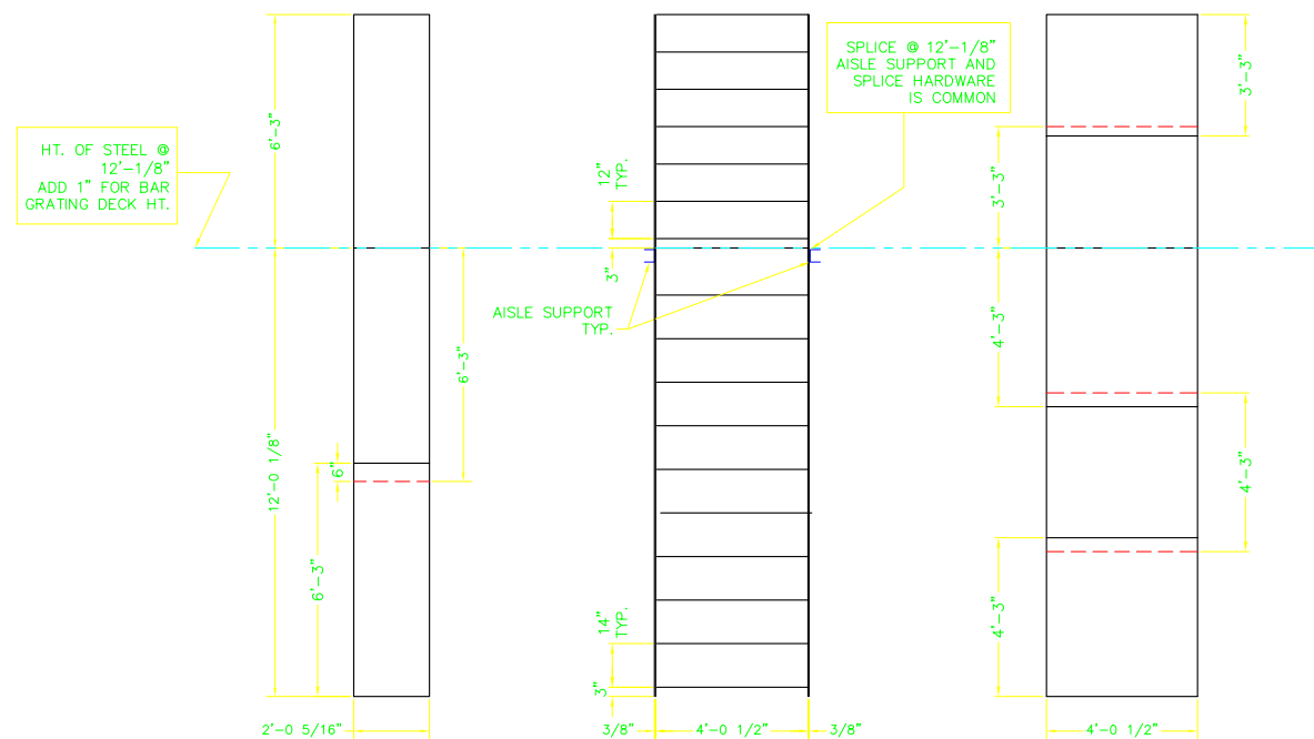
SIDE ELEVATION
