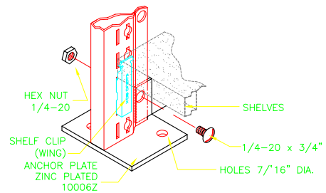
FRONT BOX POST
