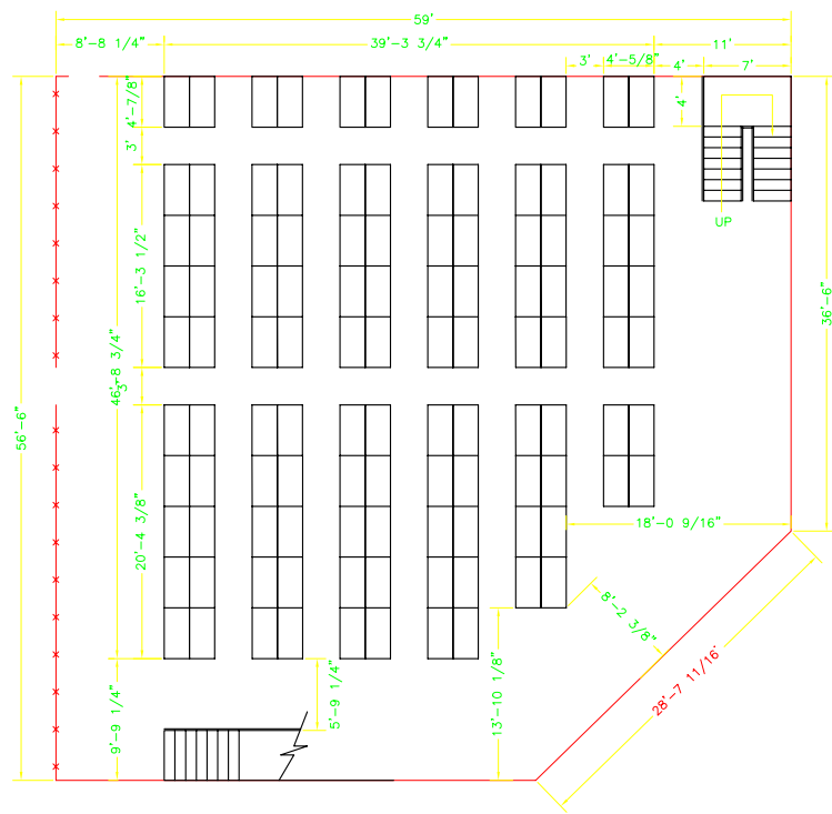
LOWER LEVEL
