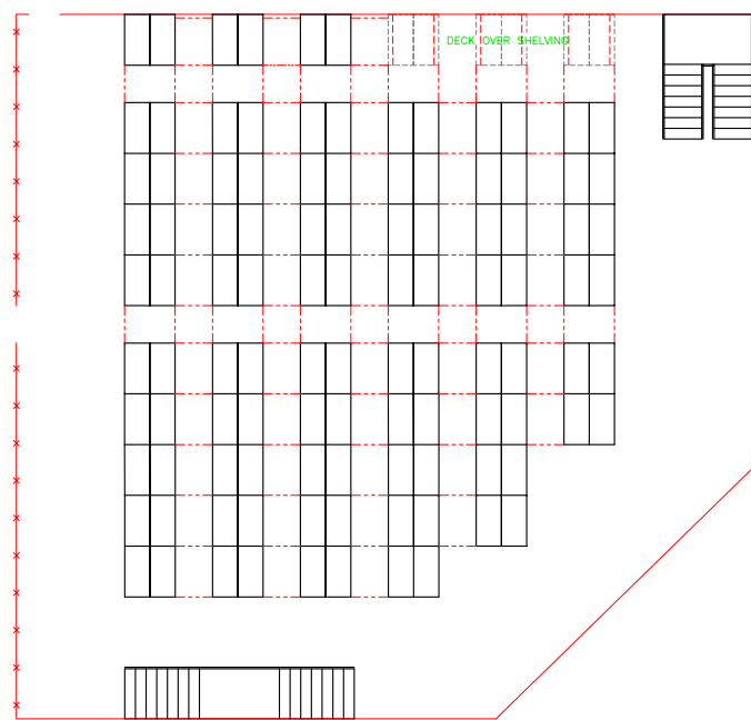
AISLE SUPPORT PLACEMENT
