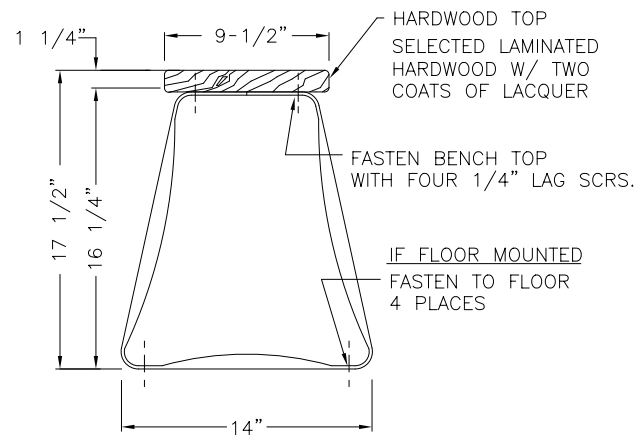
BENCH & STAINLESS STEEL PEDESTAL DETAIL
